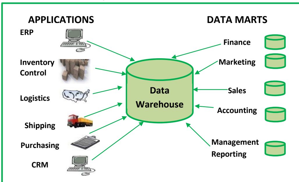
Fig. 3.3.8: Centralized view of Data Warehouse
